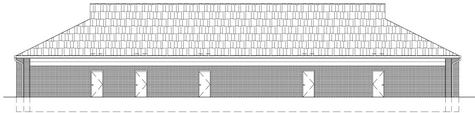
ELEVATION EAST SCALE: 1/8"=1'-0"
