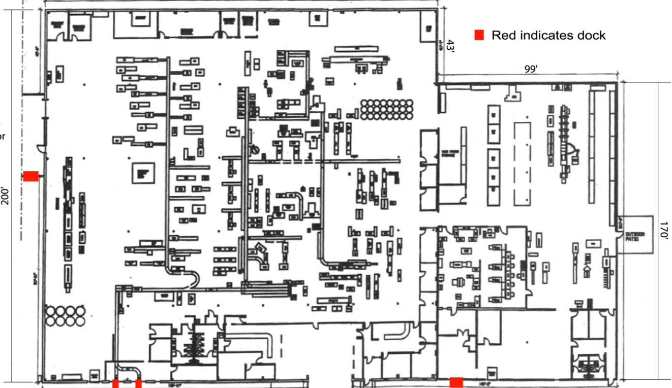
3 EXISTING RIGHT HALF OF FIRST FLOOR PLAN SCALE 1/8"=1'-0"
